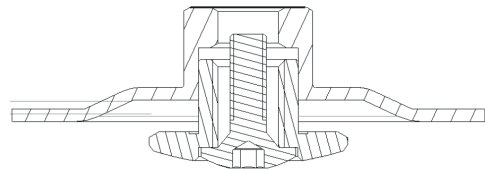
Wheel adaptor C087920 (87) with nut 6155421040 (100) and Safety screw 6156140340 (95)
