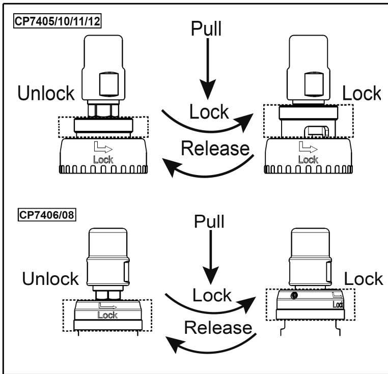
Fig. 3 Spindle Lock Instructions
